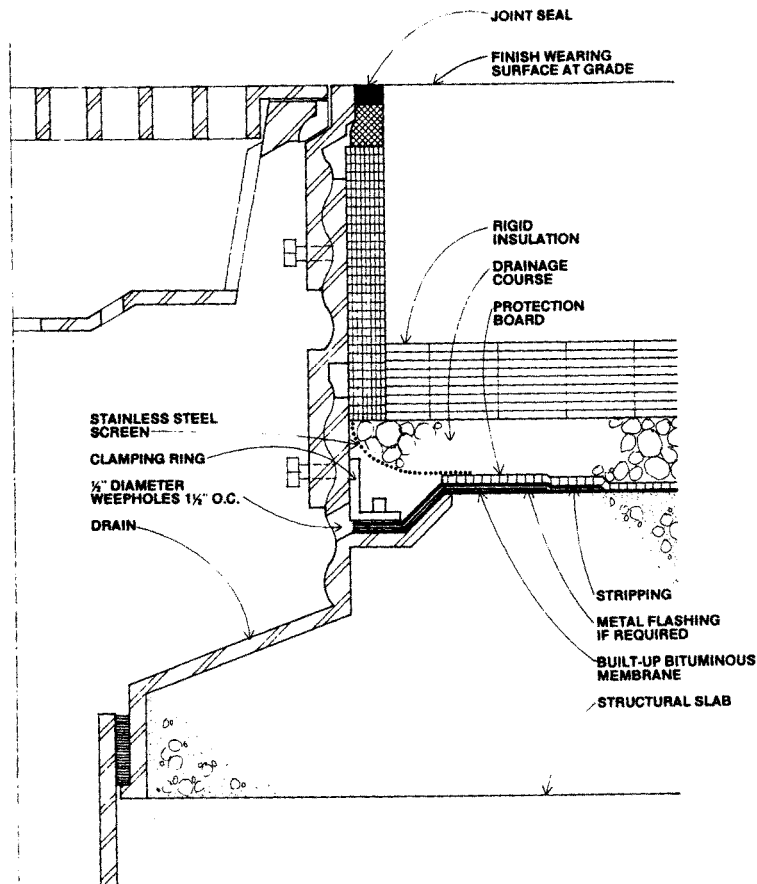
FIG. 9 Termination at Drain (see 8.8.4)
