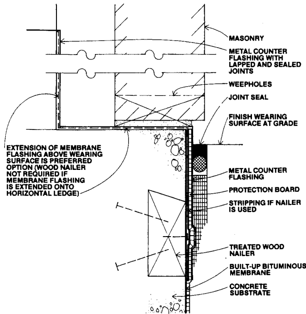
FIG. 8 Terminal Condition with Masonry Above Finish Wearing Surface at Grade (see 8.8.8 and 8.8.8.2)
