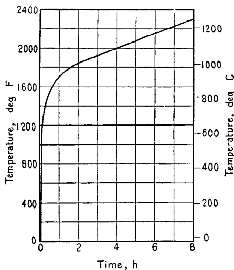
FIG. 1 Time-Temperature Curve
