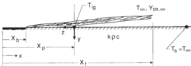
FIG. X2.1 Model for Flame Spread
