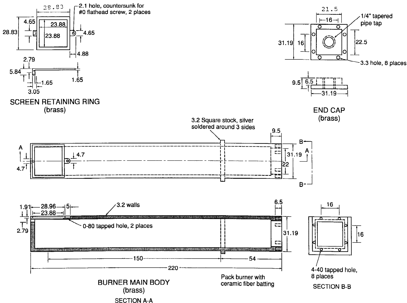
FIG. 11 Calibration Burner
