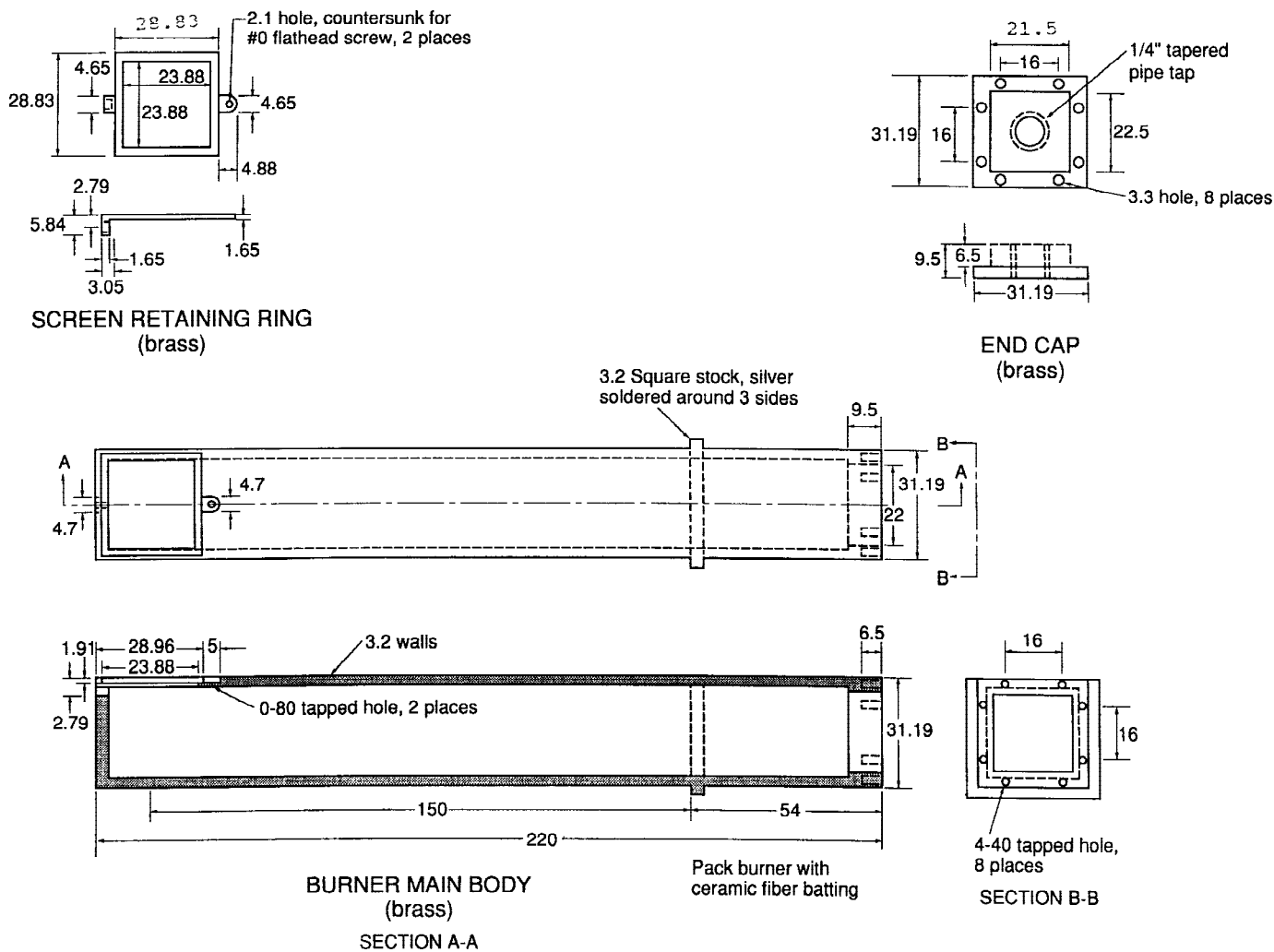
FIG. 11 Calibration Burner
