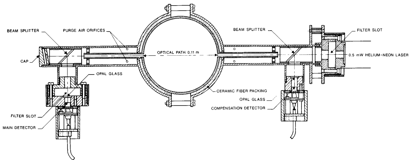
FIG. 10 Smoke Obscuration Measuring System
