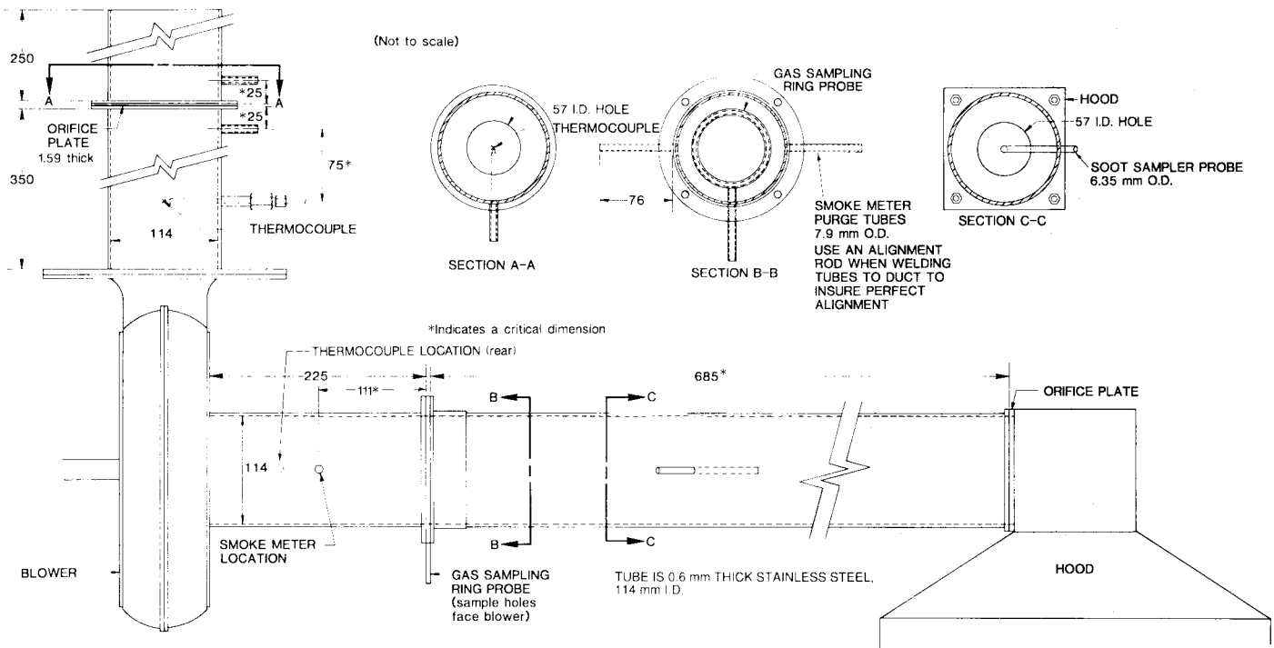
FIG. 5 Exhaust System
