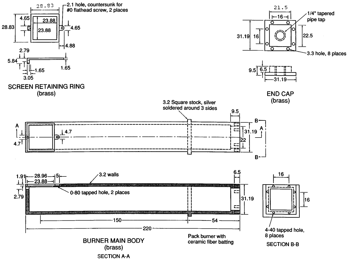
FIG. 11 Calibration Burner
