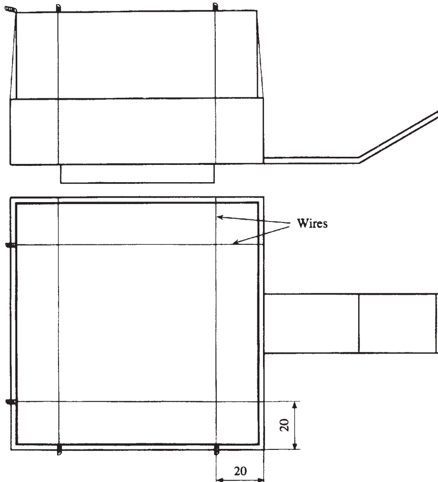
FIG. 4 Assembling of Specimen Upholstered with Leather
