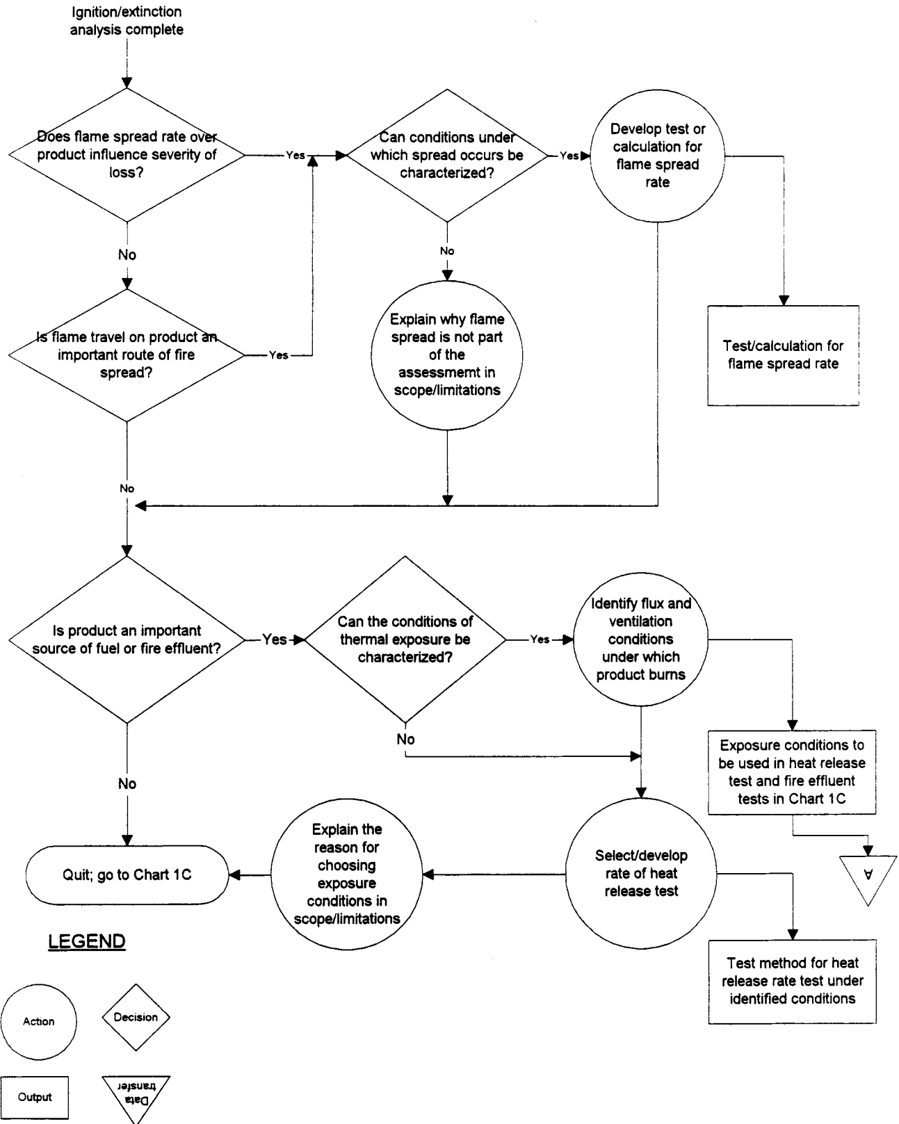
FIG. X4.3 Flow Chart 1B Flame Spread and Heat Release Ref: 8.5.2.2
