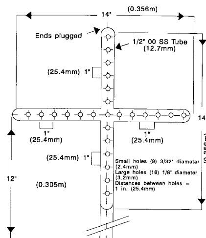
FIG. A2.3 Sampling Probe of the Cross-Shaped Type
