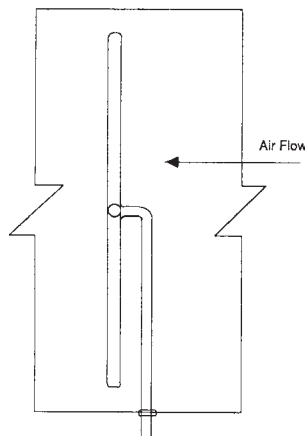
FIG. A2.3 Cross Type Sampling Probe
