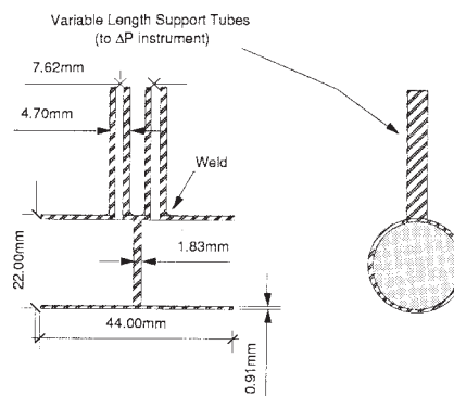
FIG. A2.1 Bidirectional Probe
