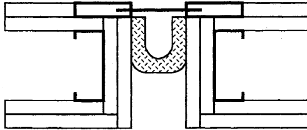
Typical Asymmetrical Wall-to-Wall Joint System
