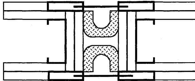
Typical Symmetrical Wall-to-Wall Joint System
