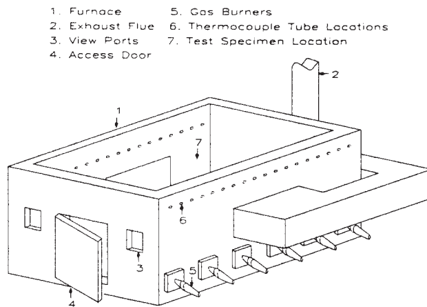
FIG. 2 Example of Horizontal Furnace
