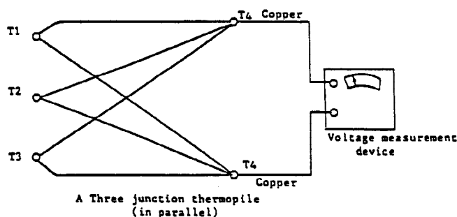
FIG. 6 Multiple-Junction Thermopiles
