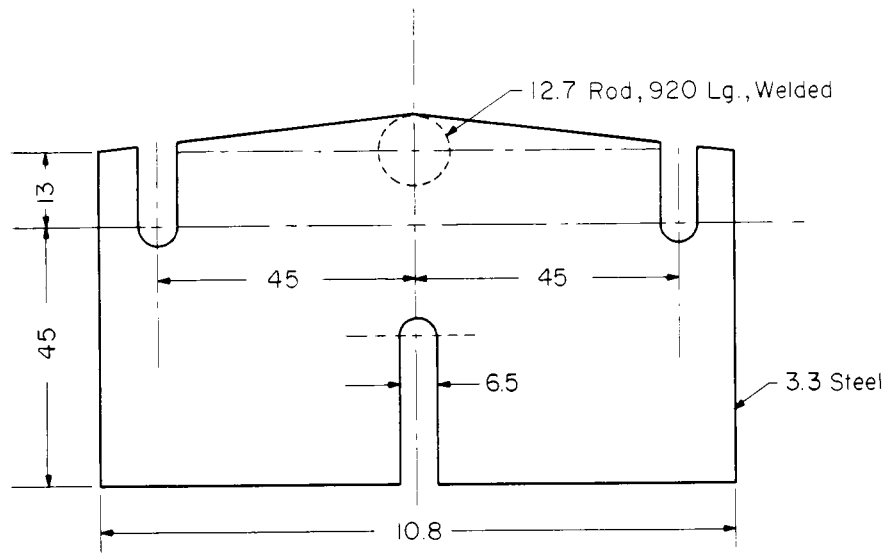
VERTICAL SUPPORT
