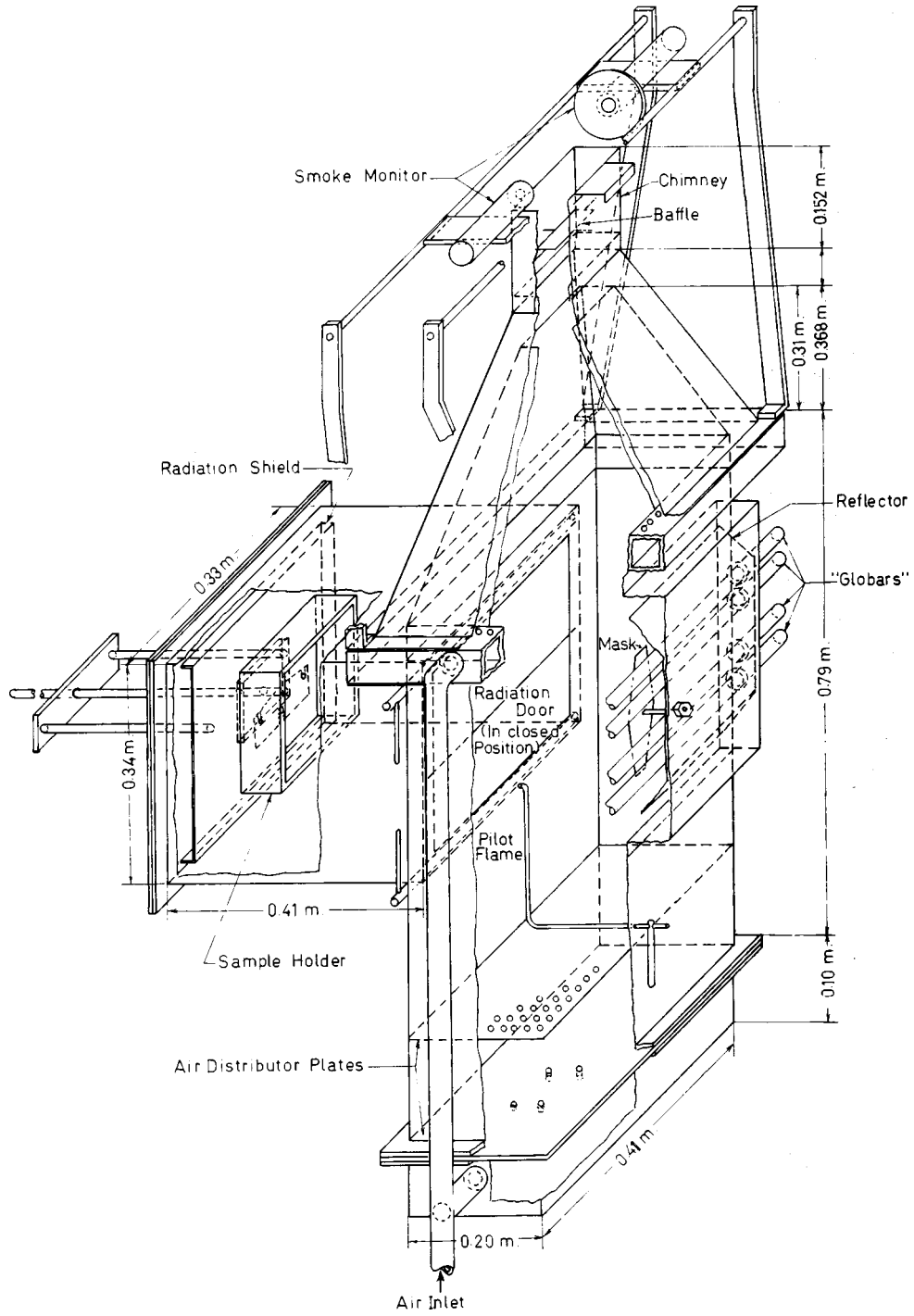
FIG. 9 Release Rate Apparatus—Configuration B
