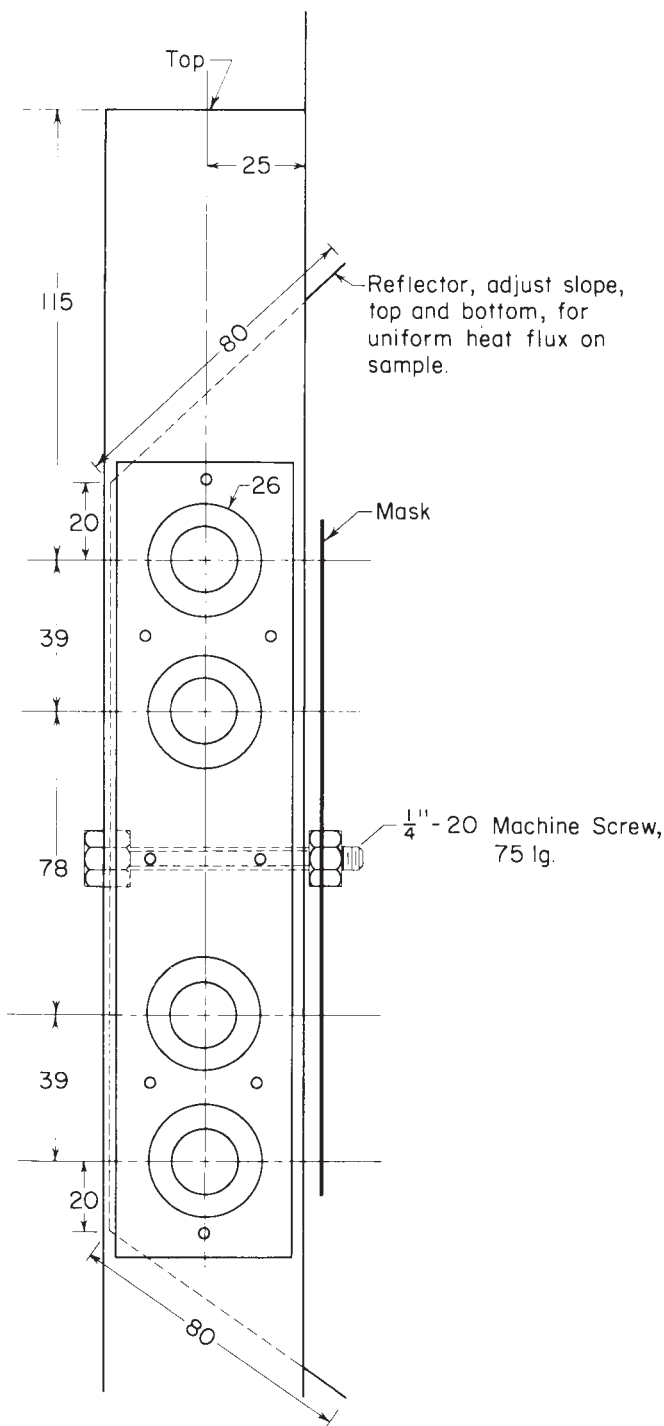
FIG. 17 Locations of Holes in Globar Radiant Panel
