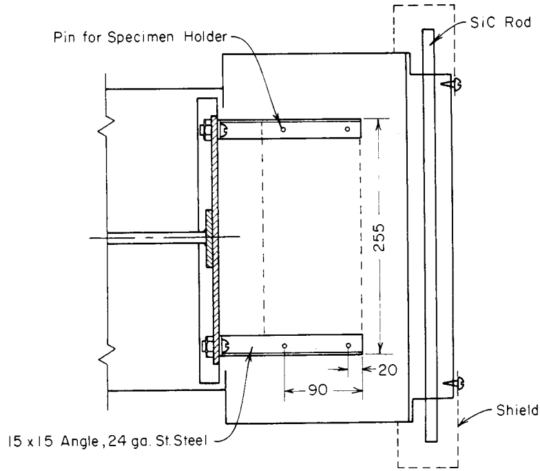
FIG. 22 Horizontal Configuration
