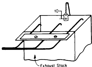
FIG. 11 Compensator Tab Mount
