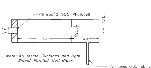
FIG. 14 Smoke Monitor
