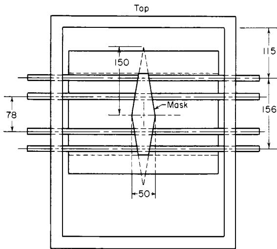
FIG. 16 Globar Radiant Panel
