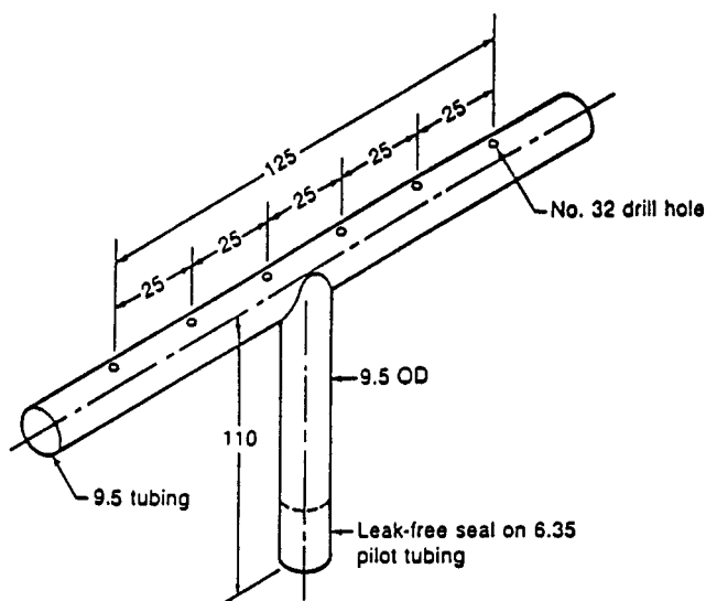
(Unless denoted otherwise, all dimensions are in millimeters.) FIG. 8 Calibration Burner—Configuration A
