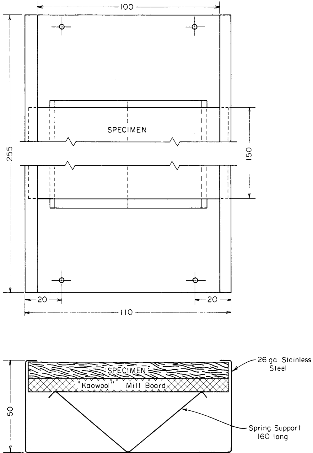
FIG. 20 Horizontal Specimen Holder
