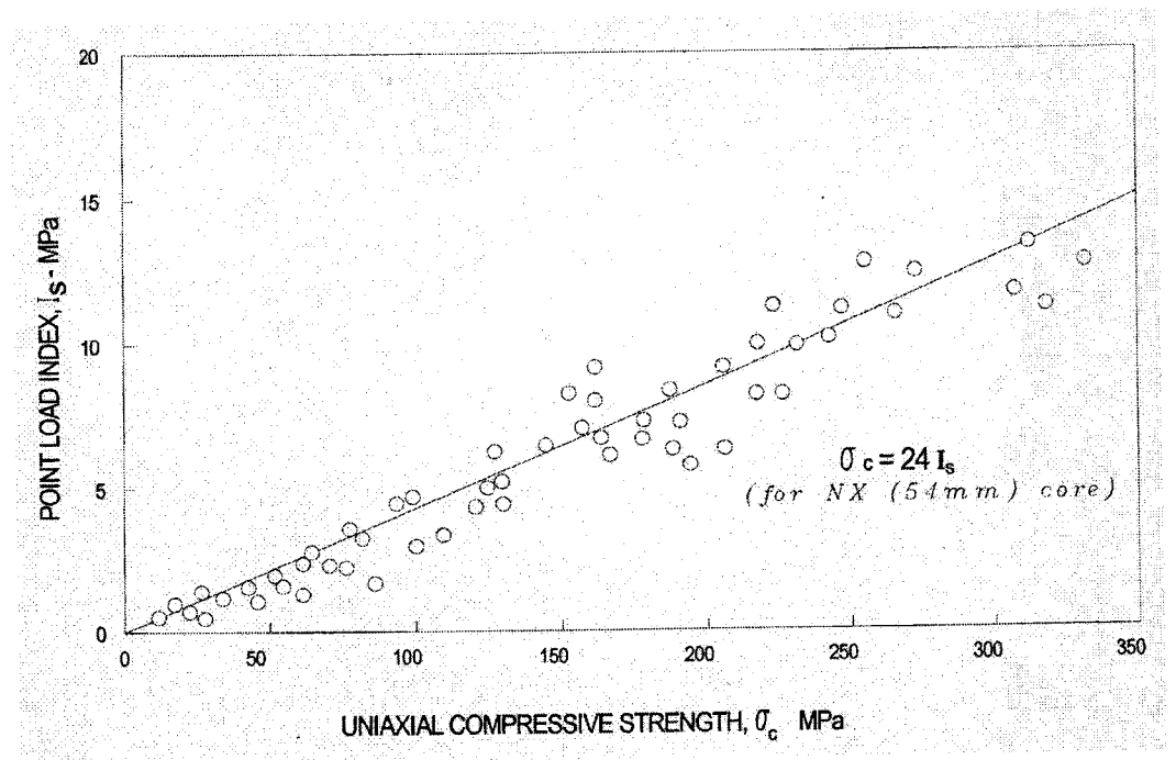
FIG. 7 Relationship Between Point Load Strength Index and Uniaxial Compressive Strength from 125 Tests On Sandstone, Quartzite, Marikana, Norite, and Belfast Norite 6
