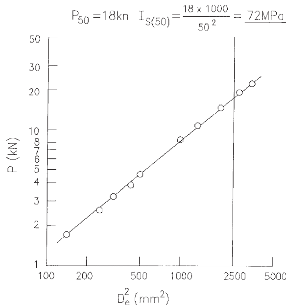
FIG. 5 Procedure for Graphical Determination of I_{s(50)} from a Set of Results at D_e Values Other Than 50 mm—(ISRM-Suggested Methods) 3, 5
