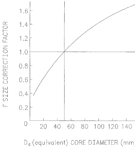
FIG. 6 Size Correction Factor Chart (ISRM Suggested Methods) 5
