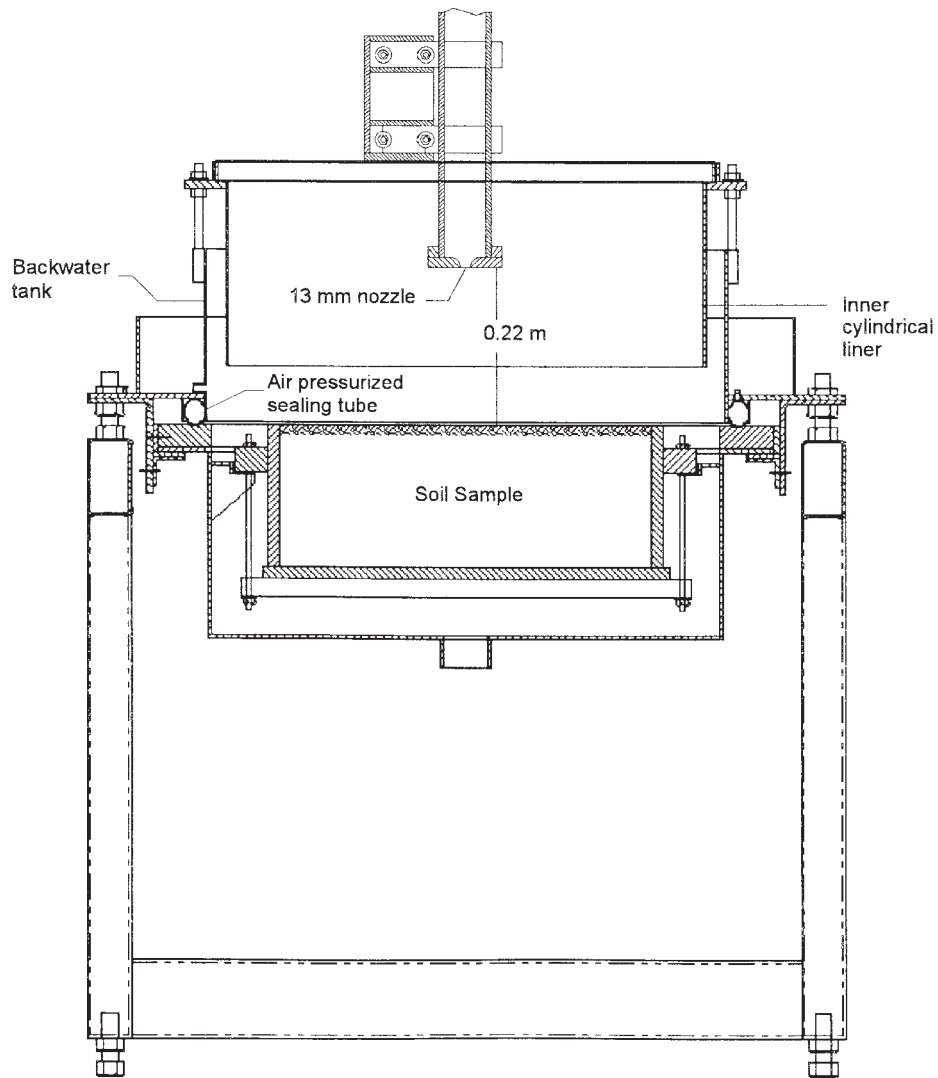
FIG. 4 Submerged Jet Apparatus for Laboratory Testing
