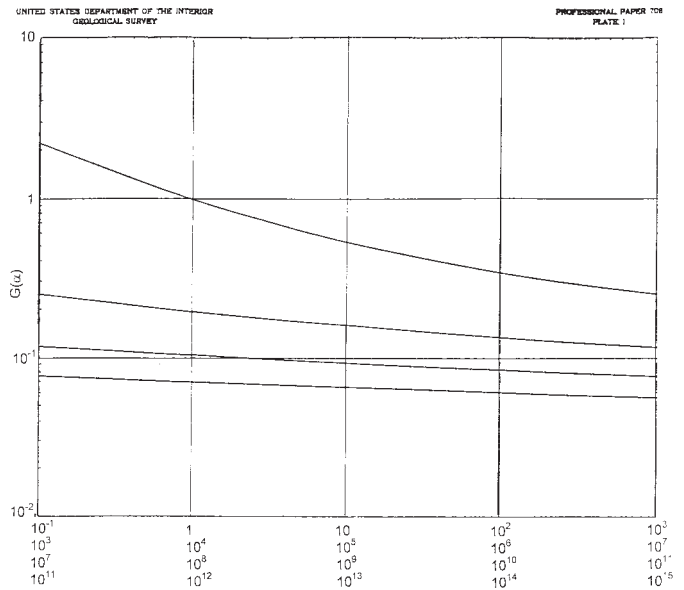
NOTE 1—After Lohman 5 , Plate 1. FIG. 2 Logarithmic Plot of \alpha Versus G(\alpha)
