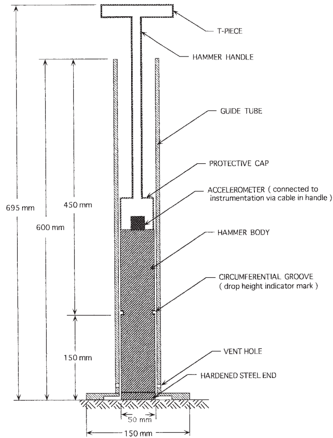
FIG. 4 Illustration (Cross Section) of a 4.5 kg Impact Soil Tester with Hammer at Rest in the Guide Tube
