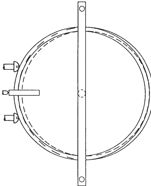
FIG. 3 Plan View of Jenike Cell Showing Offset
