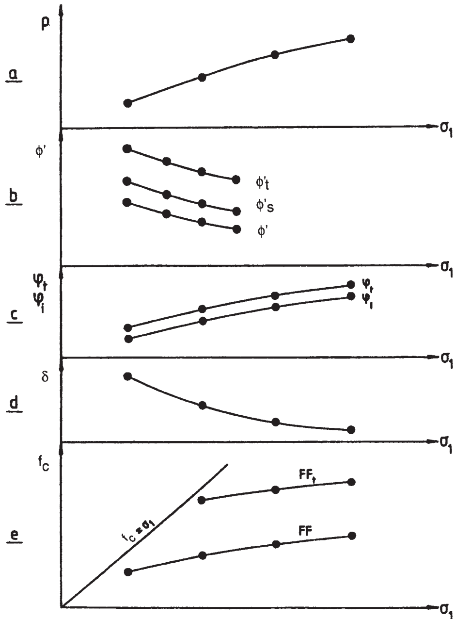
FIG. 197 Powder Properties as a Function of \sigma_1
