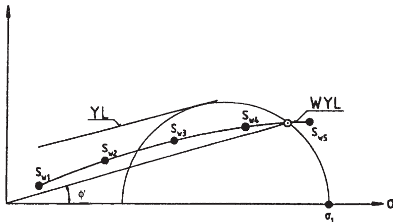
FIG. 189 Wall Yield Locus
