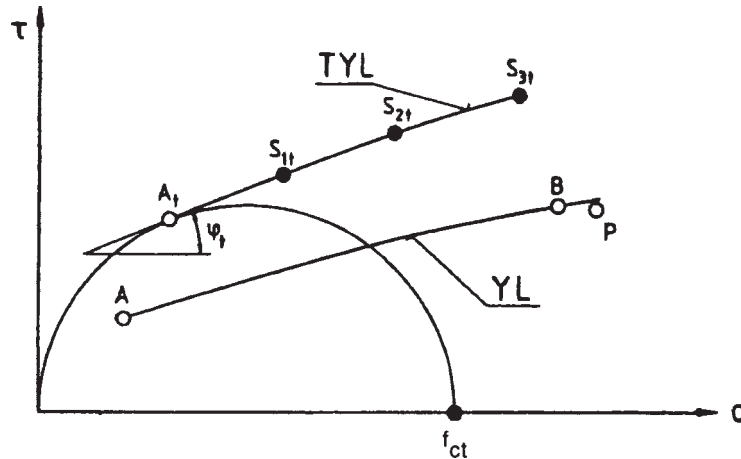
FIG. 178 Time Yield Locus
