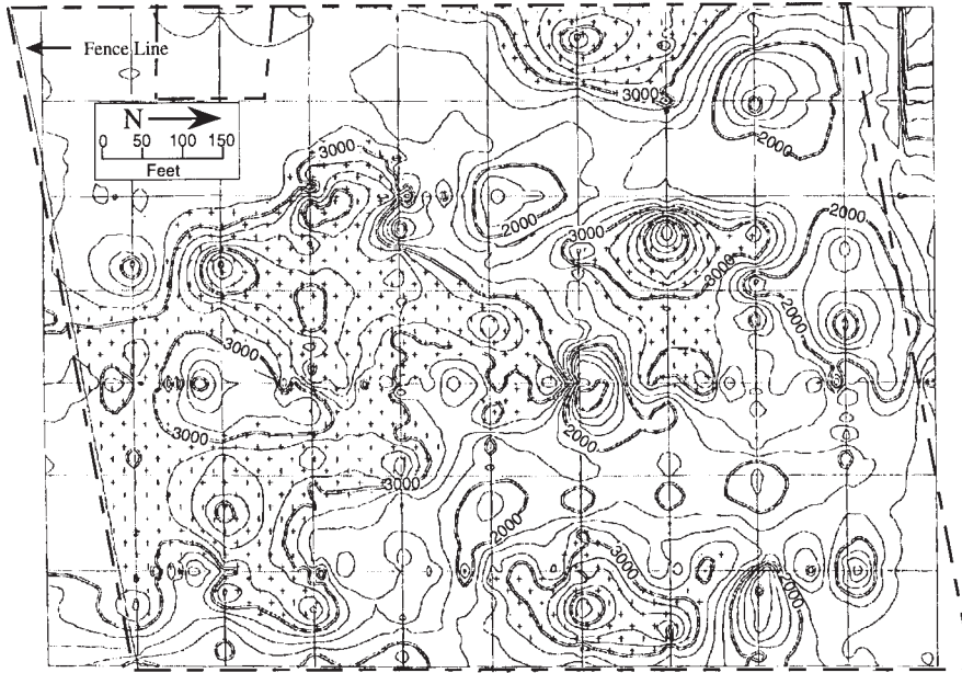
NOTE 1—Values are in gammas. Areas 200 gammas above background are marked with + symbol and represent solid waste trench locations. FIG. X6.1 Total Field Magnetic Contour Map for Flora Vista Landfill
