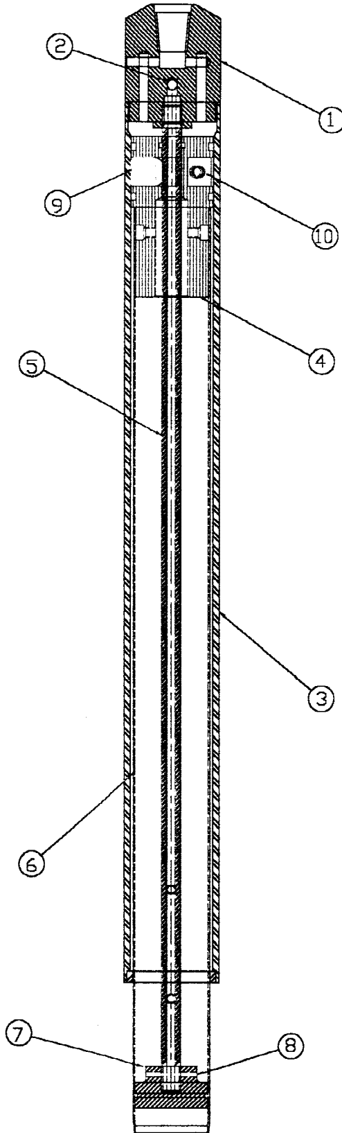
FIG. 2 Hydraulically Operated Stationary Piston Sampler
