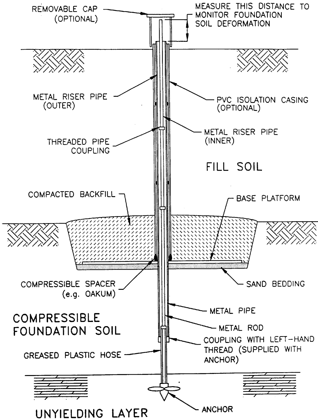
FIG. 3 Typical Installation for Internally Referenced Settlement Platform with Borros Anchor
