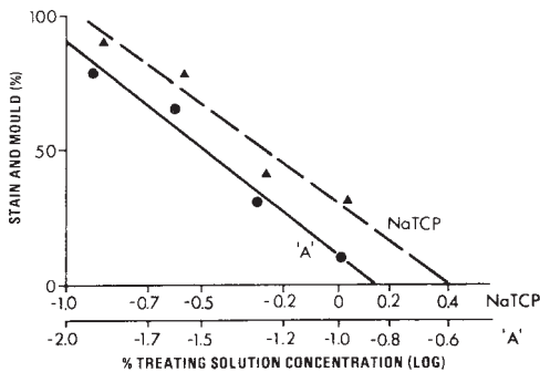
FIG. 3 Example of CGo Determination for Unknown Chemical A, Compared with Sodium Tetrachlorophenate (NaTCP). CGo for NaTCP is About 2.5 % and for Fungicide A is About 0.13 % (see 14.2.5)
