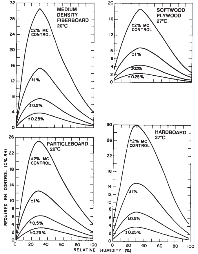
FIG. X1.2 Relative Humidity Control Required to Maintain EMC of Composite Wood Products with Required Limits
