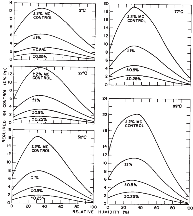
FIG. X1.1 Relative Humidity Control Required to Maintain EMC of Solid Wood with Required Limits
