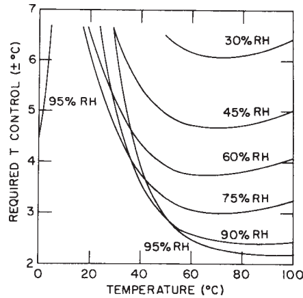
FIG. X1.3 Temperature Control Required to Maintain EMC of Solid and Composite Wood Products within \pm 0.25\% MC (Ref (6))
