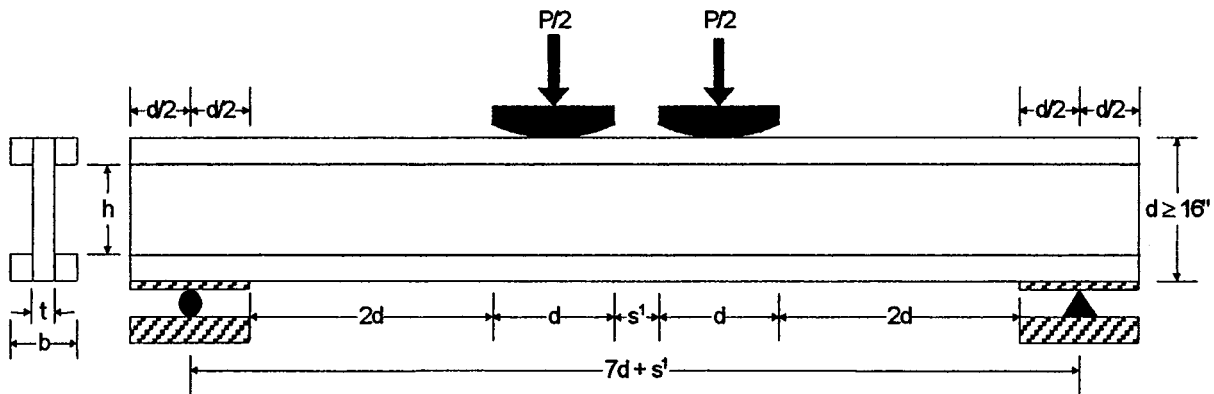
FIG. A3.2 Example LVL Structural-Size Horizontal Shear Test Set-Up
