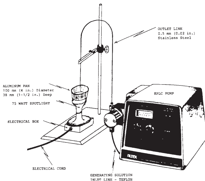
FIG. X2.1 Equipment Description
