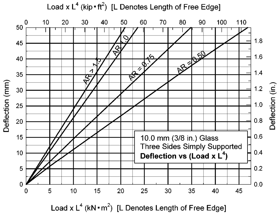
FIG. A1.20 (upper chart) Nonfactored Load Chart for 10.0 mm (3/8 in.) Glass with Three Sides Simply Supported (lower chart) Deflection Chart for 10.0 mm (3/8 in.) Glass with Three Sides Simply Supported
