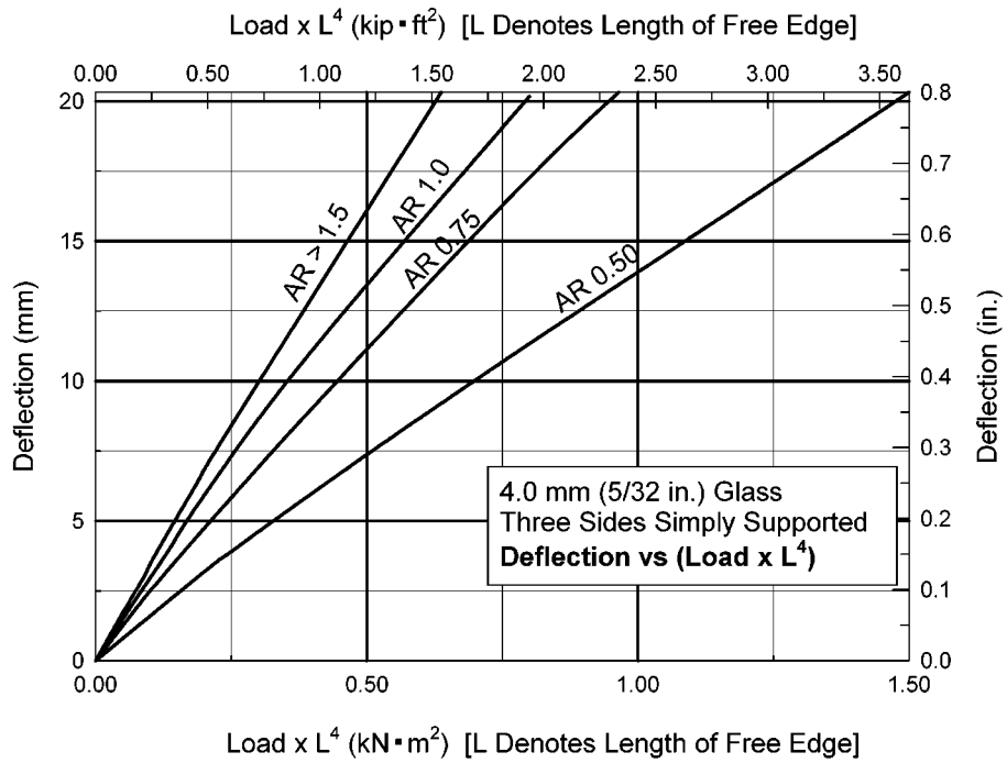
FIG. A1.16 (upper chart) Nonfactored Load Chart for 4.0 mm (5/32 in.) Glass with Three Sides Simply Supported (lower chart) Deflection Chart for 4.0 mm (5/32 in.) Glass with Three Sides Simply Supported
