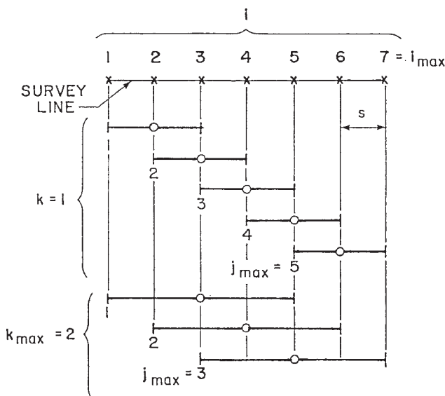
FIG. X1.1 Chord Positions
