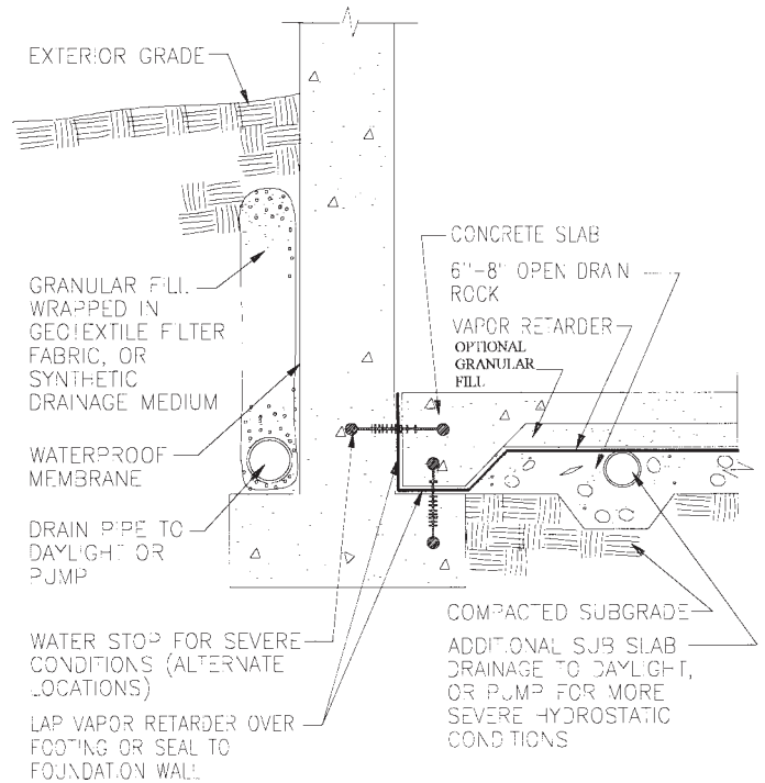
FIG. 3 Concrete Slab on Grade: Solution for Subgrade Up to One Story below Grade with No Hydrostatic Pressure on Vapor Retarder
