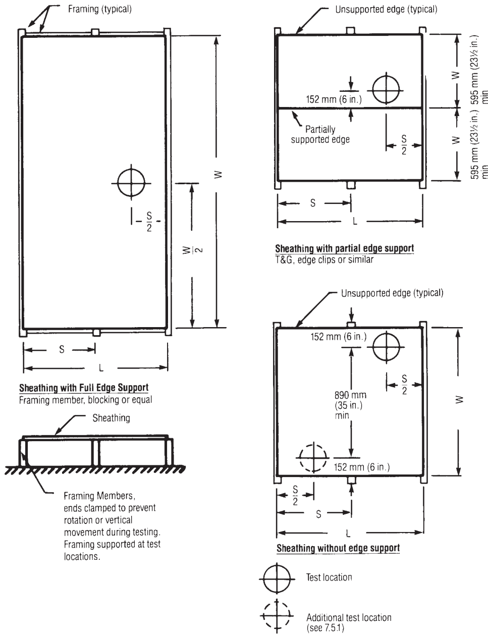
FIG. 4 Impact-Load Test Specimens
