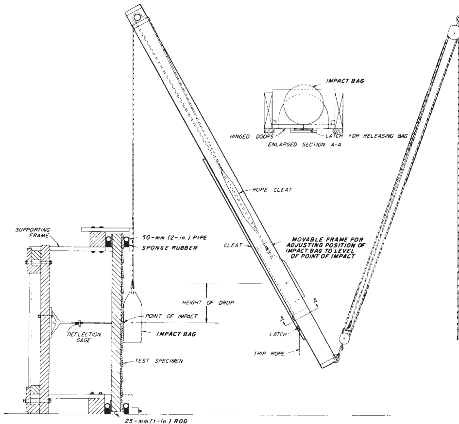
FIG. 2 3 Impact Load Test (Specimen Vertical)
