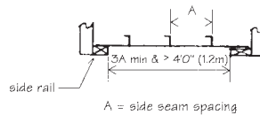
section "x"
