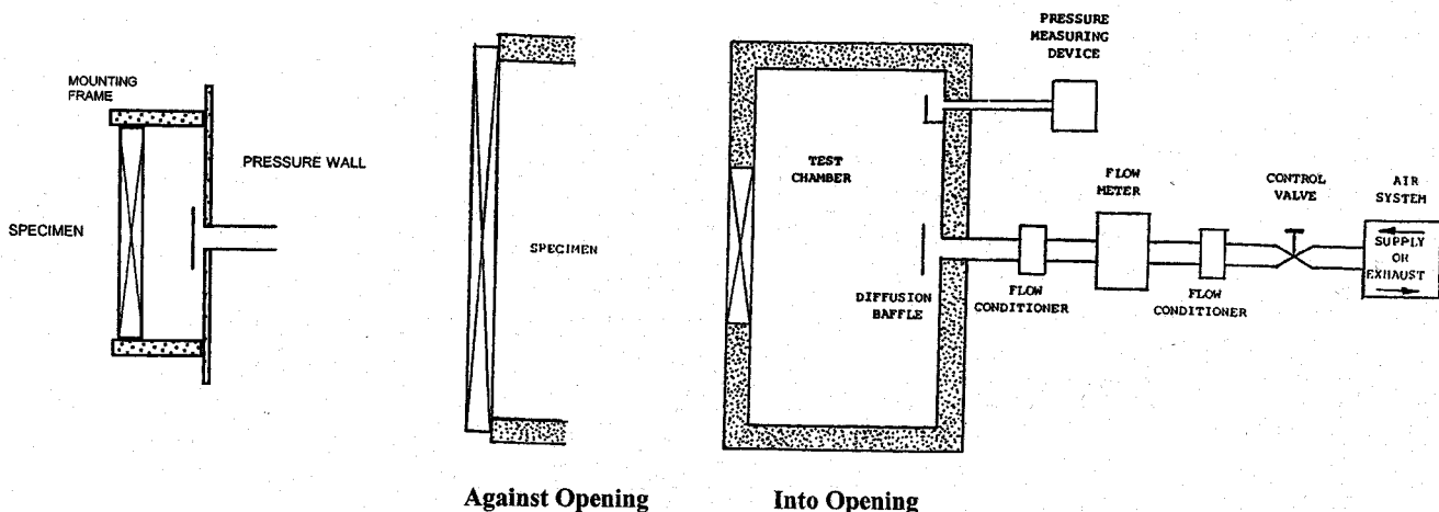
FIG. 1 General Arrangement of the Air Leakage Apparatus
