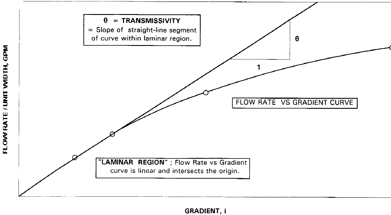
FIG. X1.1 Hydraulic Transmissivity
