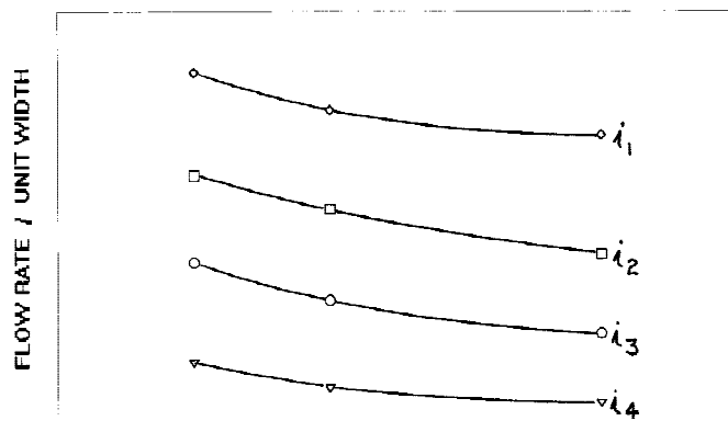
NORMAL COMPRESSIVE STRESS FIG. 3 Typical Plot of Flow Rate per Unit Width Versus Normal Compressive Stress at Several Hydraulic Gradients
