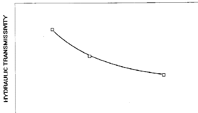
NORMAL COMPRESSIVE STRESS FIG. 4 Typical Plot of Hydraulic Transmissivity Versus Normal Compressive Stress
