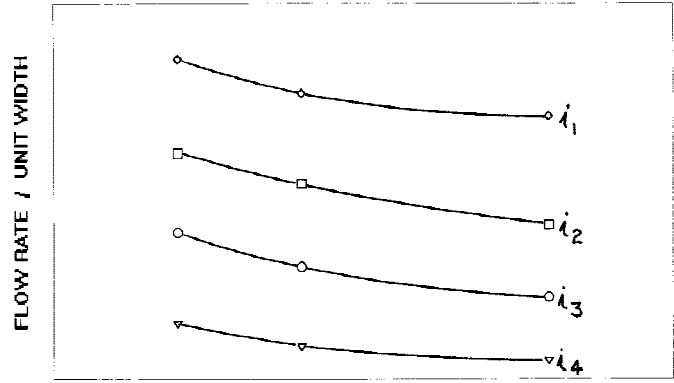
FIG. 3 Typical Plot of Flow Rate per Unit Width Versus Normal Compressive Stress at Several Hydraulic Gradients
