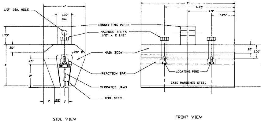
FIG. X2.4 Sanders Clamp
