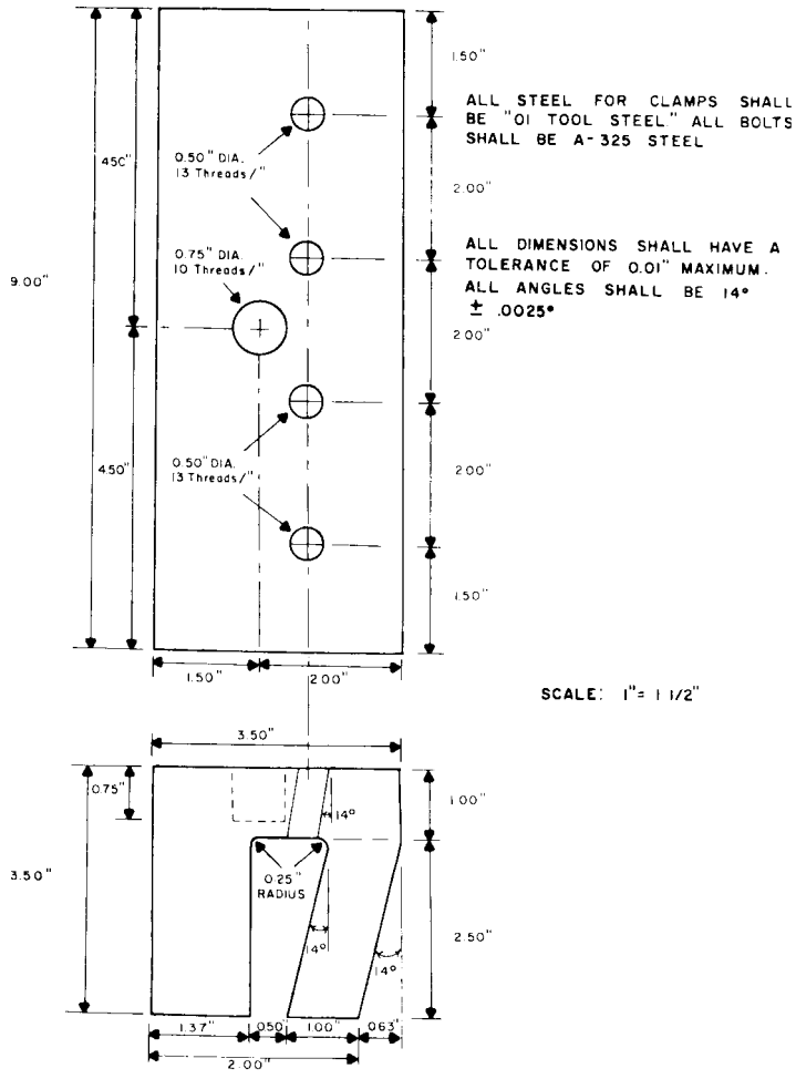
WIDE WIDTH TEST CLAMPS (MAKE 2 CLAMPS)
