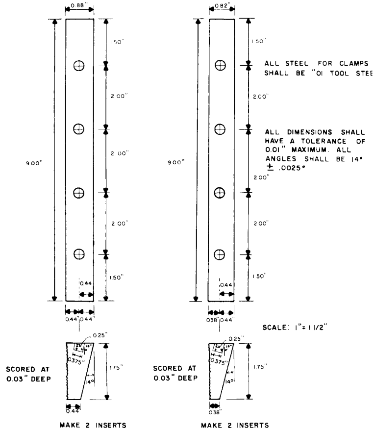
FIG. X2.2 Inserts for Wide Width Clamps
