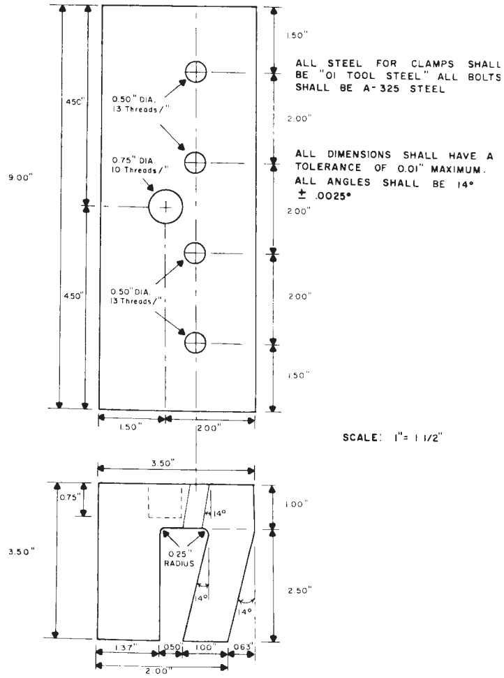
WIDE WIDTH TEST CLAMPS (MAKE 2 CLAMPS)
