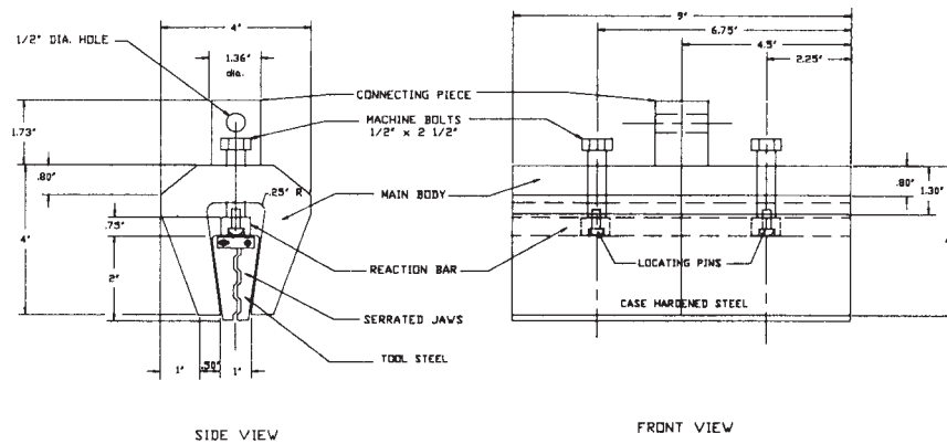
FIG. X2.4 Sanders Clamp
