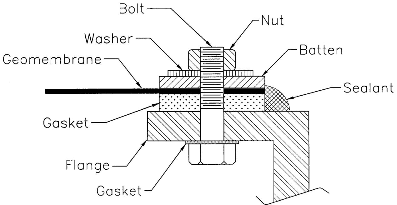
FIG. 12 Batten Attachment to Flange
