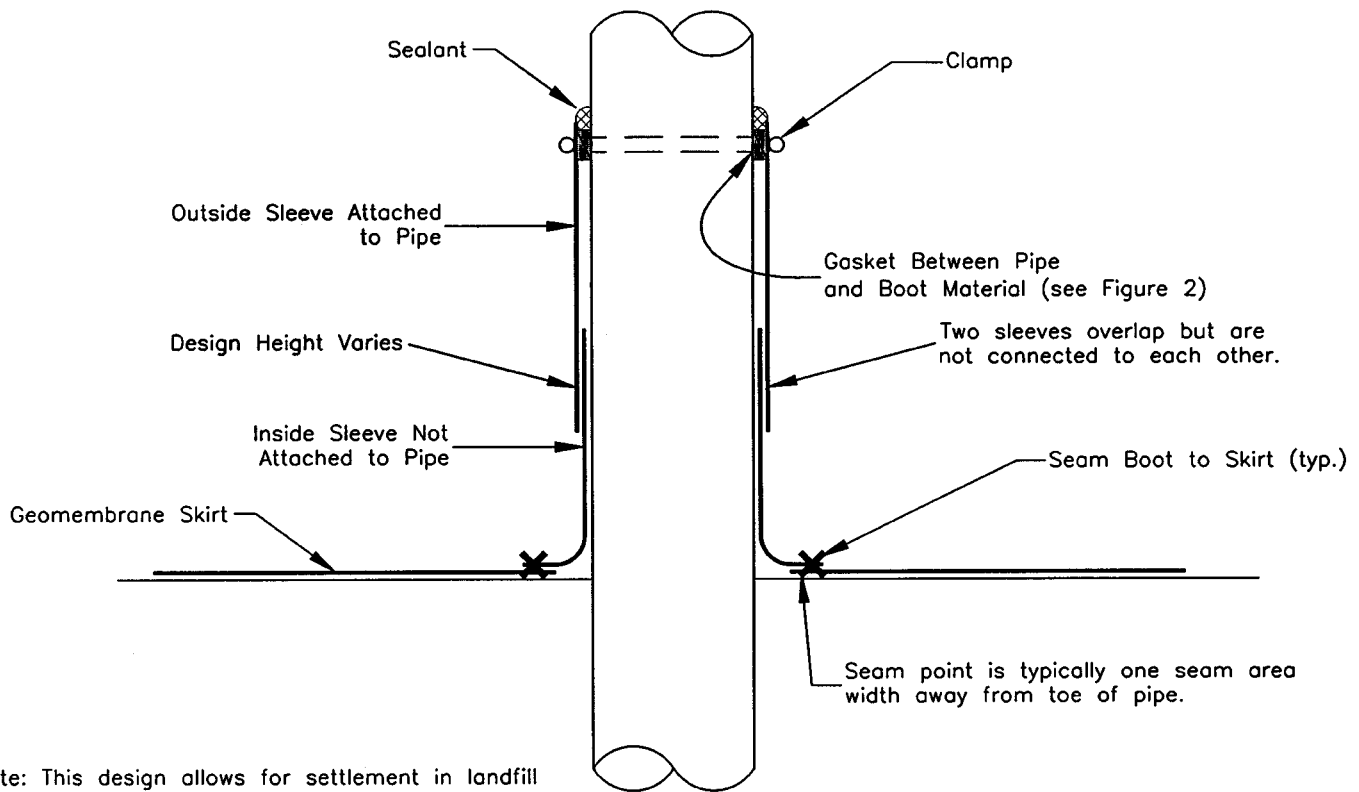
FIG. 14 Slip Boot Detail
