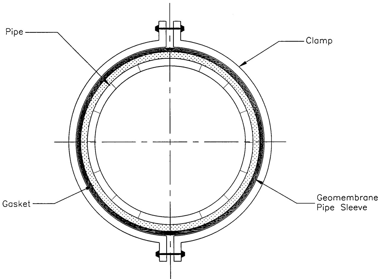
FIG. 2 Clamp Detail
