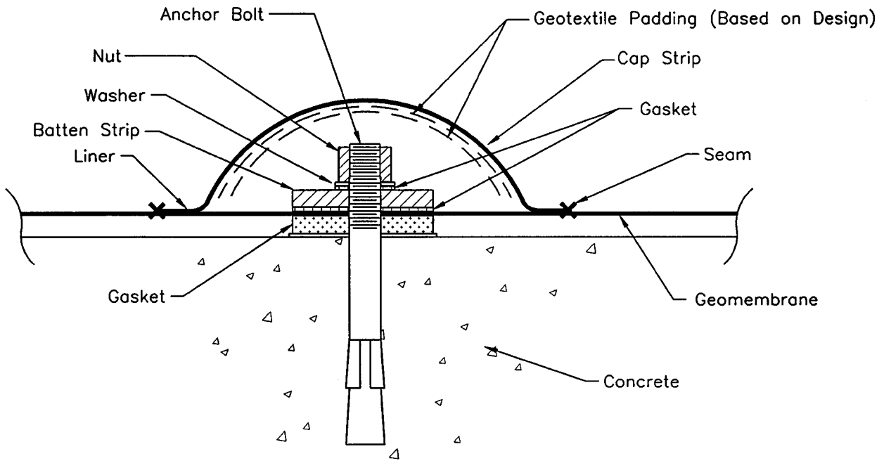
FIG. 8 Batten Attachment with Cap Strip
