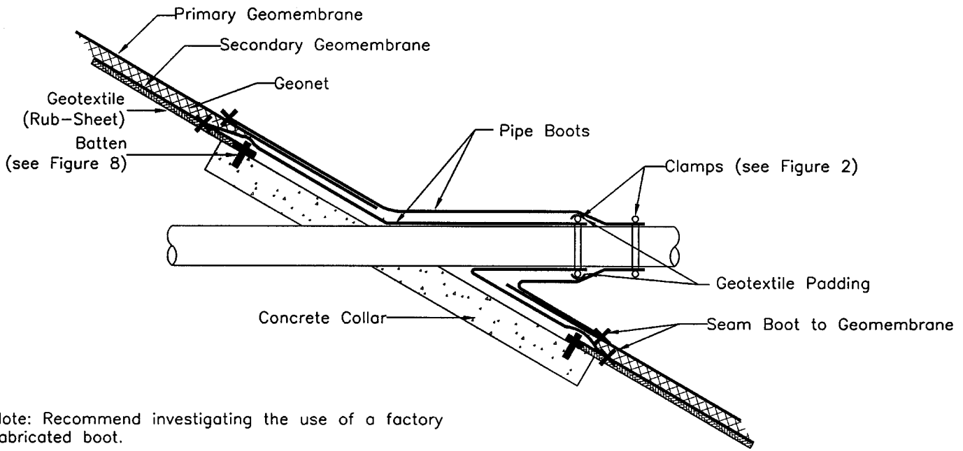
FIG. 9 Pipe Penetration—Double Layer System with Collar
