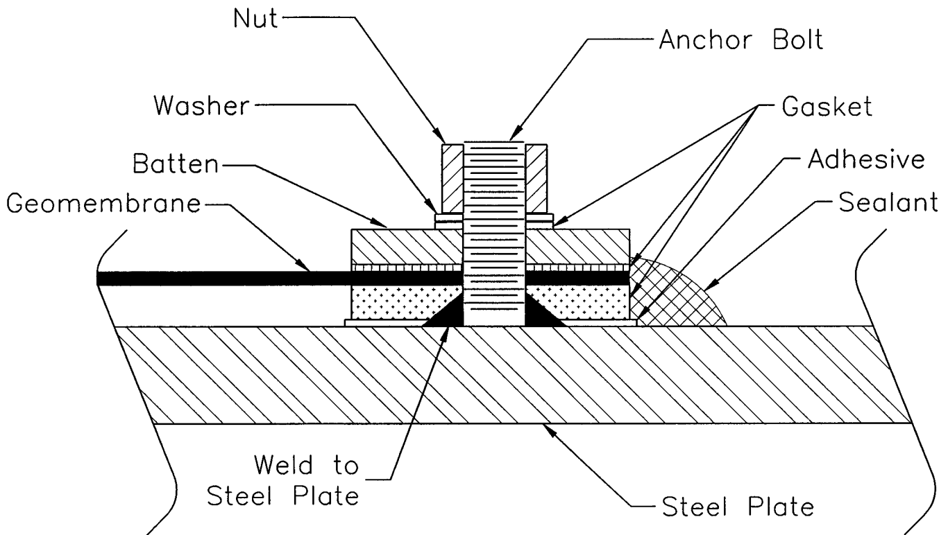
FIG. 10 Batten Attachment to Steel Plate
