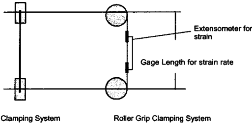
FIG. 3 Gage Length For Fixed and Roller Grip Clamping Systems
