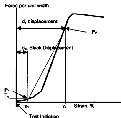
FIG. 4 Stress-Strain Curve with Complete Test Results
