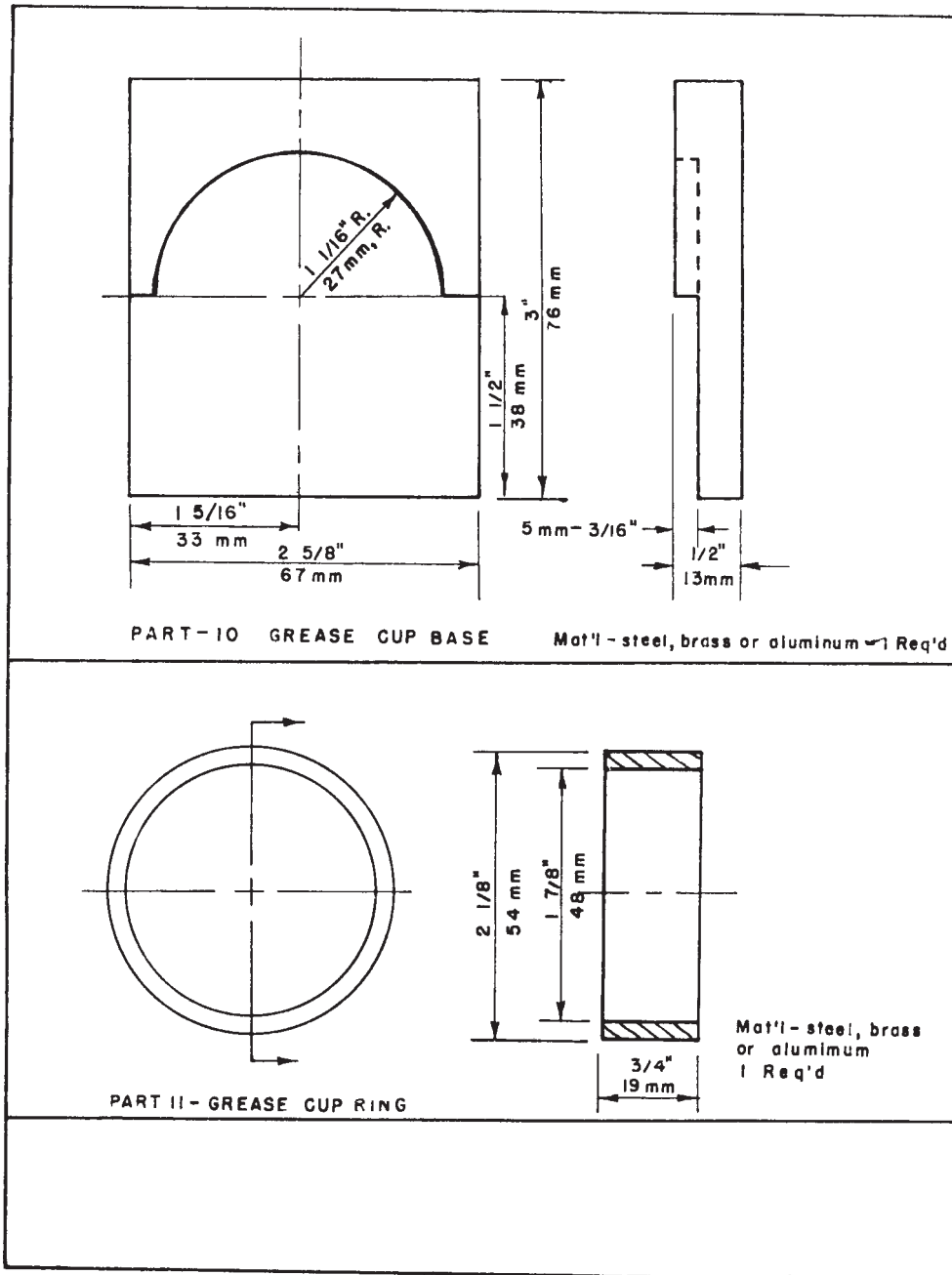
FIG. 5 Grease Cup
