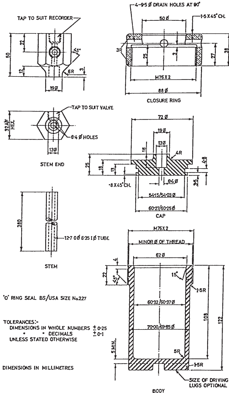
FIG. A1.4 Details of Oxidation Vessel
