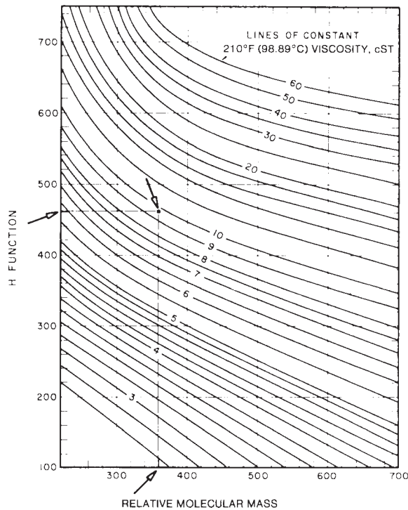
FIG. 1 Viscosity-Mean Relative Molecular Weight Mass Chart
