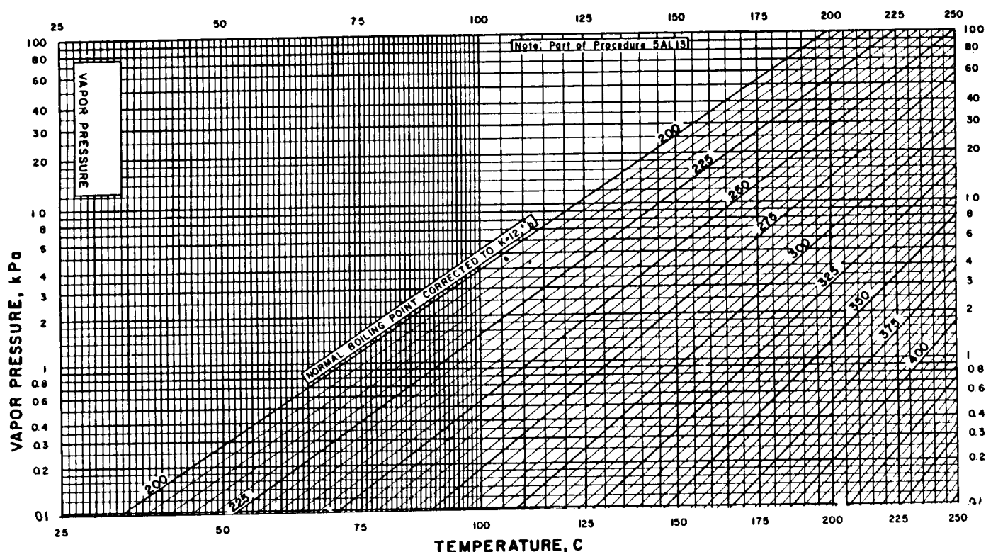
FIG. 4 Vapor Correction Chart
