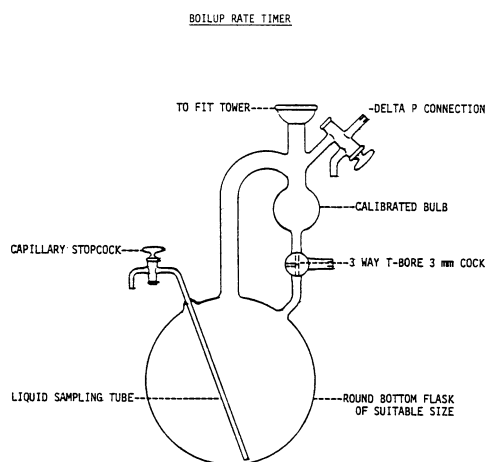
FIG. A1.2 Boiling Rate Timer
