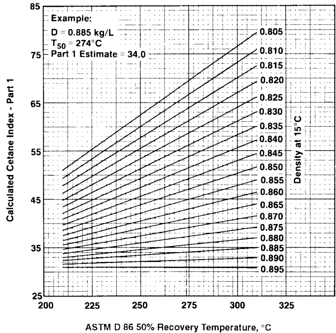
ASTM D 86 50% Recovery Temperature, °C FIG. 1 Calculated Cetane Index
