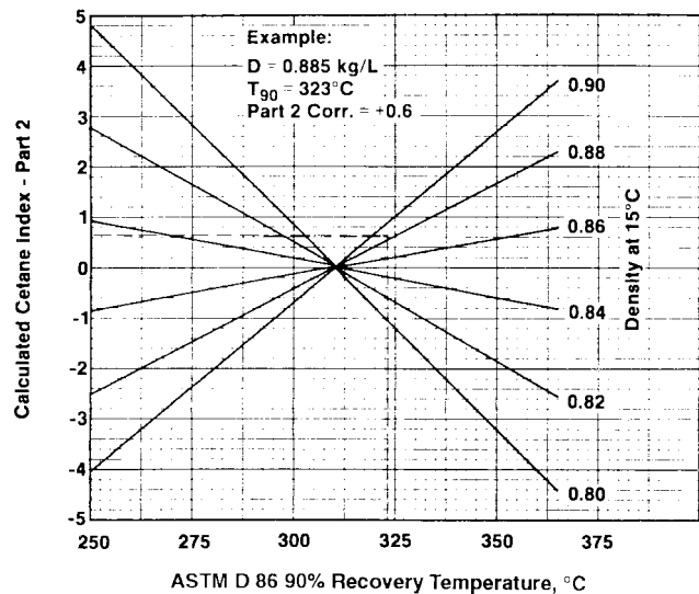
ASTM D 86 90% Recovery Temperature, °C FIG. 2 Calculated Cetane Index
