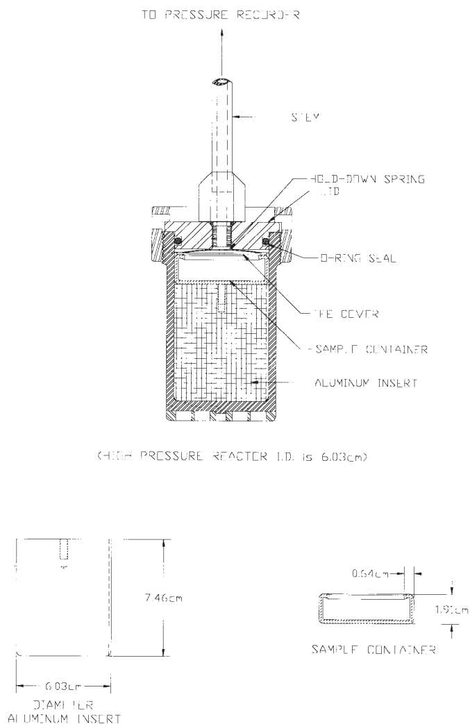
FIG. 3 2 Schematic Drawing of an Assembled Bomb, Aluminum Insert, and Glass Sample Container
