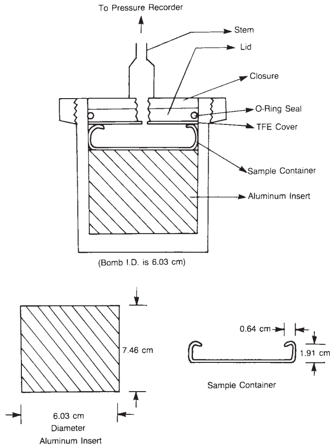
FIG. 2.1 Schematic Drawing of Oxidation Test Apparatus
