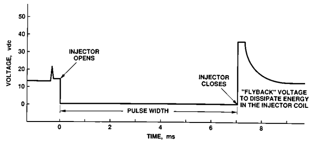
FIG. A3.45 Typical Ford EEC-IV Pulse Width
