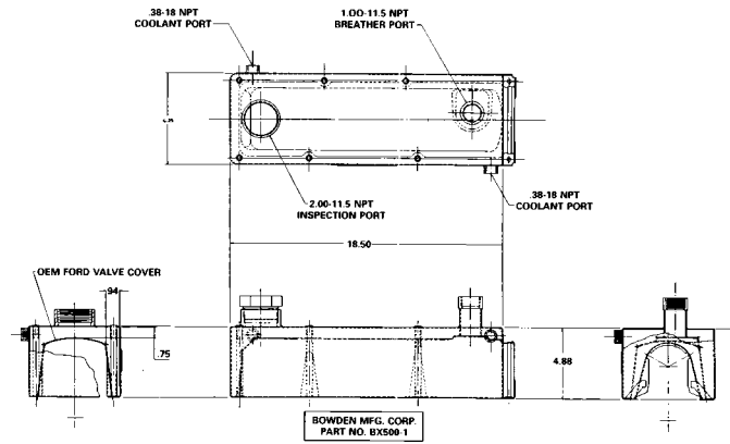
FIG. A3.26 Heated and Cooled Rocker Cover Modification
