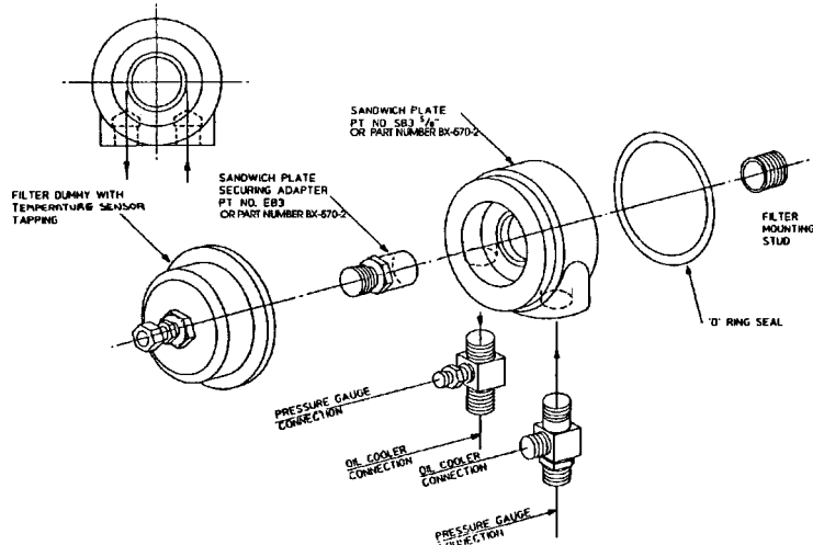
FIG. A3.39 Modified Oil Filter Sandwich Plate With Dummy Filter
