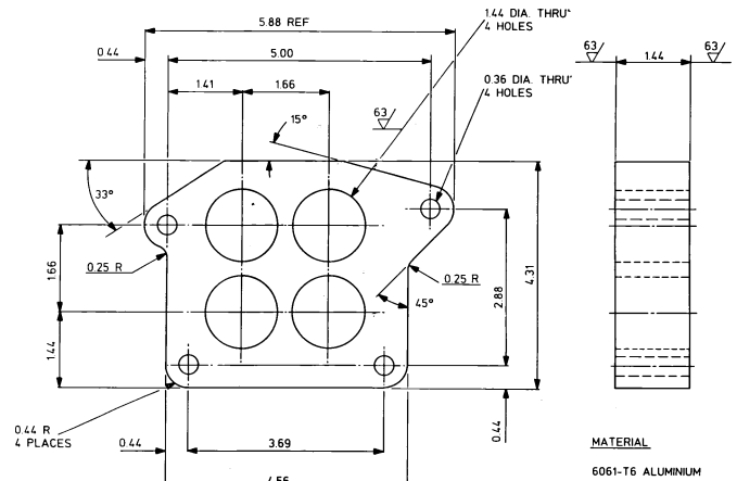
FIG. A3.20 Intake Manifold Spacer
