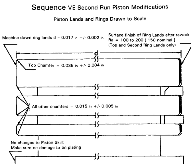
FIG. A15.1 One-half Millimetre Oversize Piston Modifications
