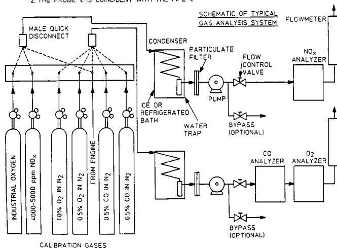
FIG. 3 Exhaust System and Exhaust Gas Analysis Apparatus
