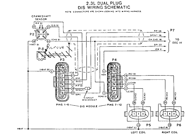
FIG. A3.48 Modifications to Distributorless Ignition System Wiring Harness
