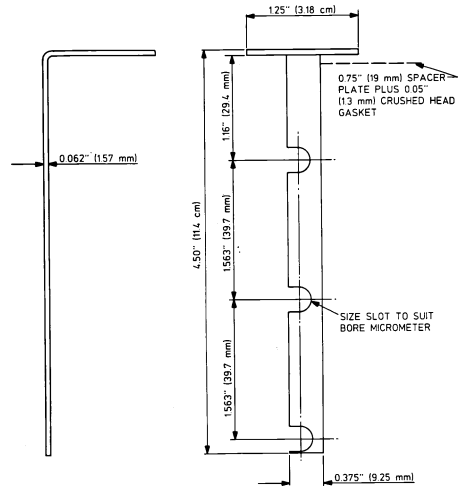
FIG. A3.38 Positioning Ladder for Bore Micrometer
