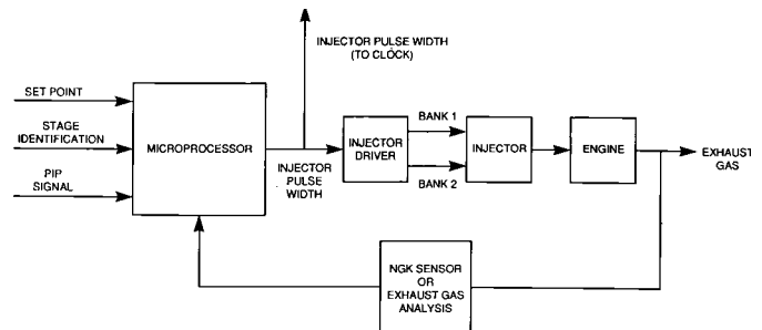
FIG. A3.23 Schematic Drawing of Closed-Loop Fuel Management System
