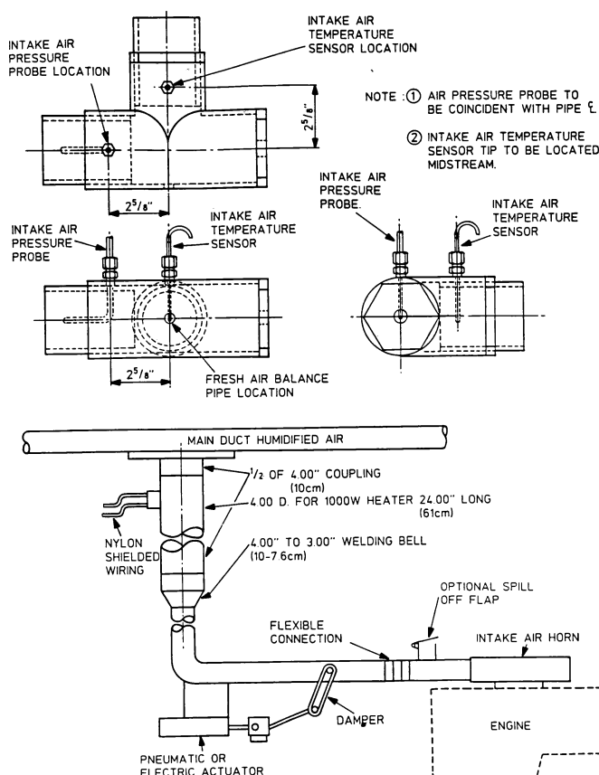
FIG. 1 Intake-Air Horn Adapter and Typical Test Stand Air Supply Duct
