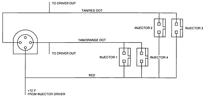
FIG. A3.44 Schematic Diagram of Injector Wiring Harness
