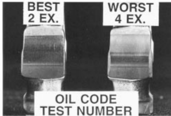
FIG. A7.18 Front Seal Housing and Rocker Arm Photographs
