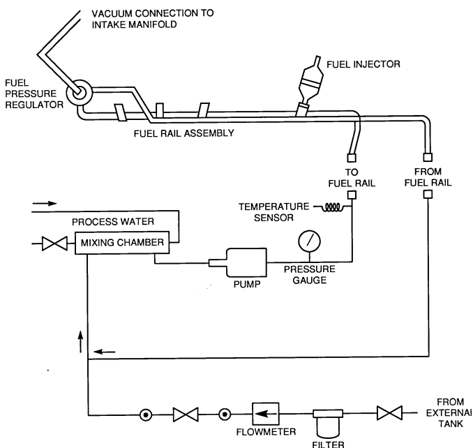
FIG. 4 Schematic of Engine Fuel System
