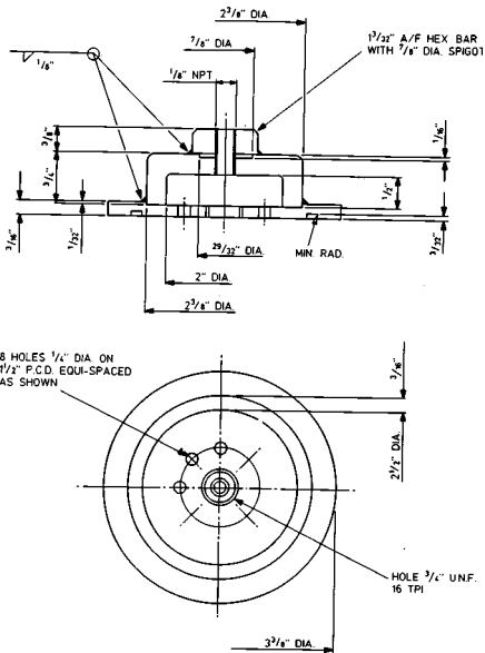
FIG. A3.40 Dummy Filter
