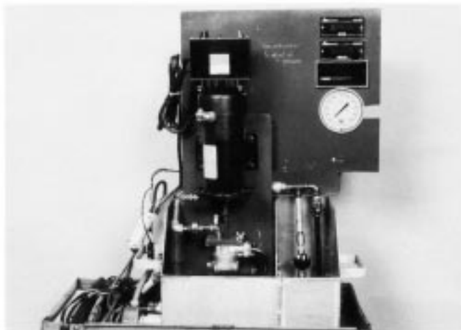
FIG. A3.31 Oil Pump Calibration Apparatus
