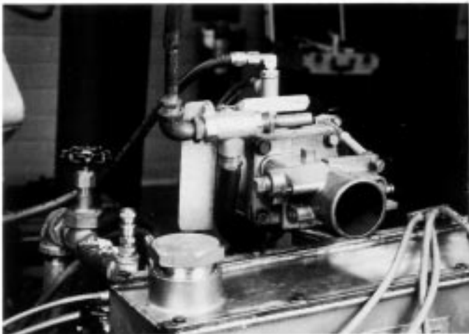
FIG. A3.18 Engine Ventilation System, Three-Way Valve
