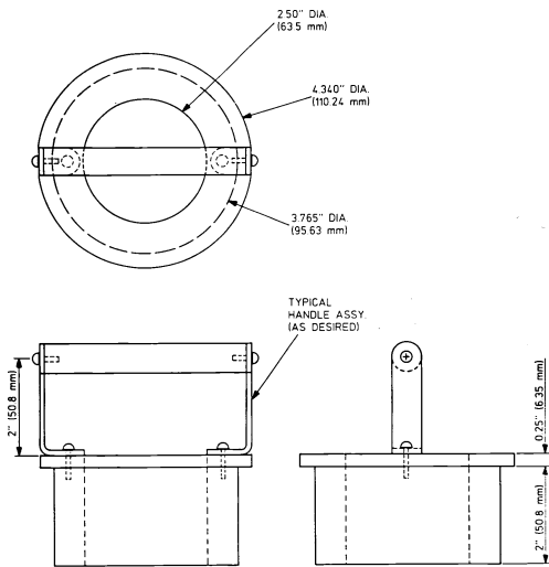
FIG. A3.36 Cylinder Block Stress Plate
