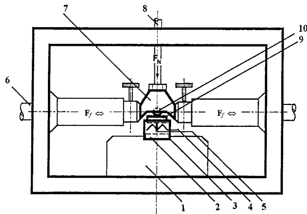
FIG. 2 Test Chamber
