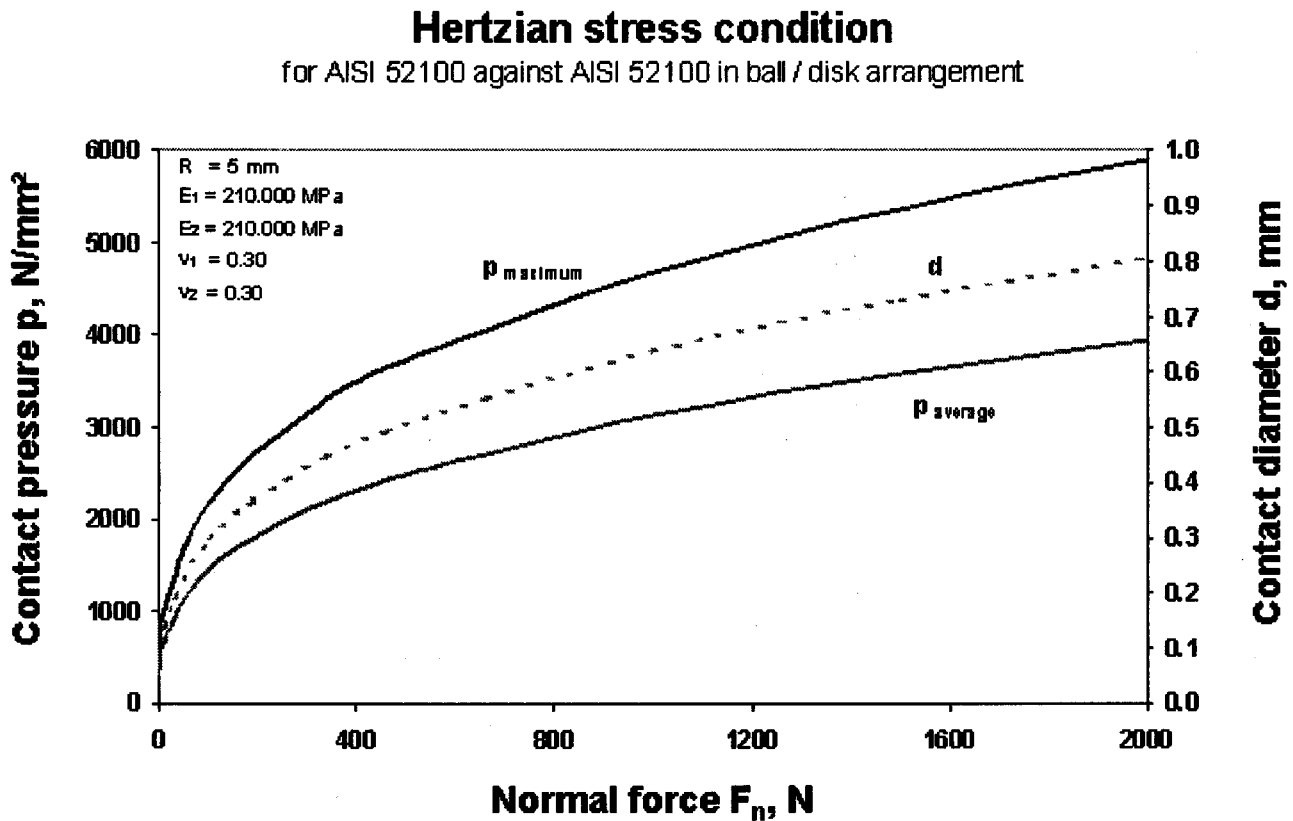
FIG. 6 Evaluation of Hertzian Contact Diameter and Contact Pressure over Test Load
