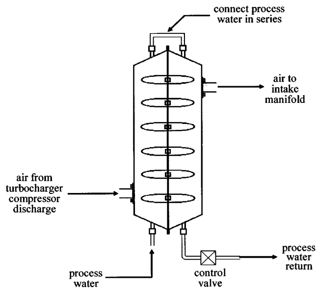
NOTE—Process water connections can be reconfigured for laboratory convenience. FIG. A4.9 After Cooler Assembly
