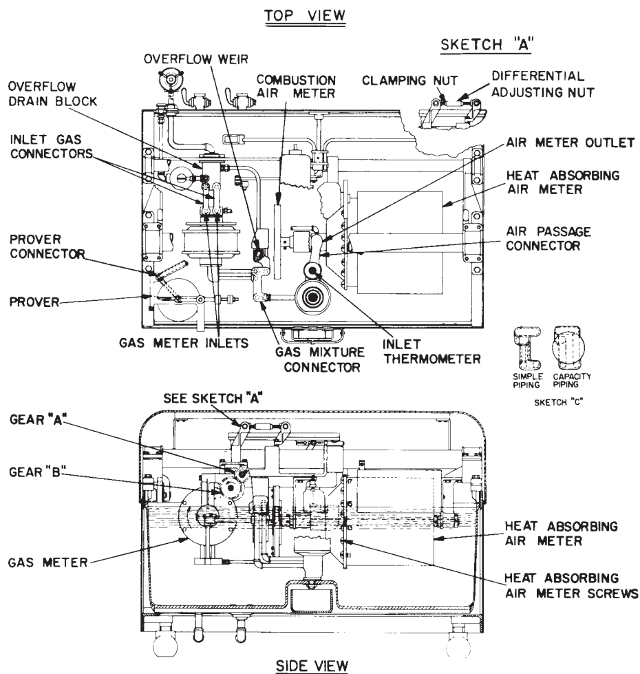
FIG. 2 Calorimeter—Layout Diagram
