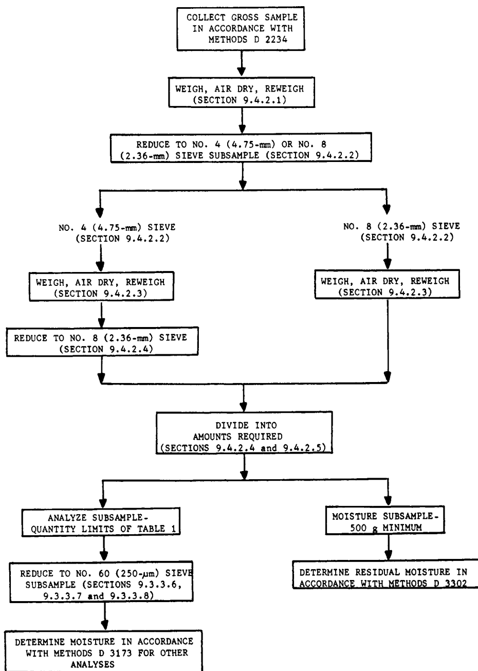
FIG. 2 Gross Sample Preparation for Moisture Determination (Referee Method)
