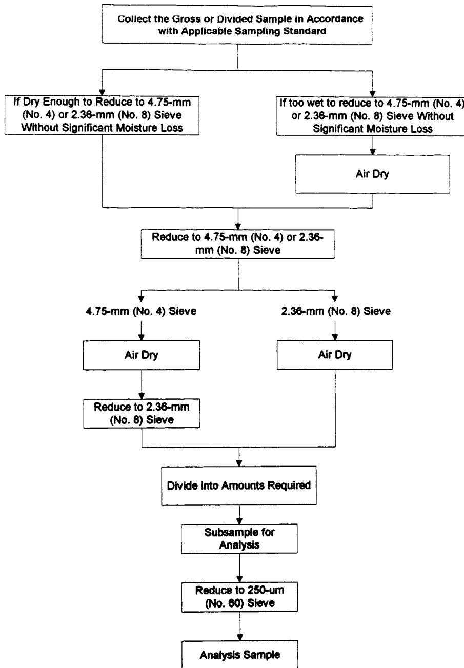
FIG. 3 Gross Sample Preparation Flowchart
